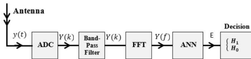
Figure 5: Block diagram of ANN location outline.
