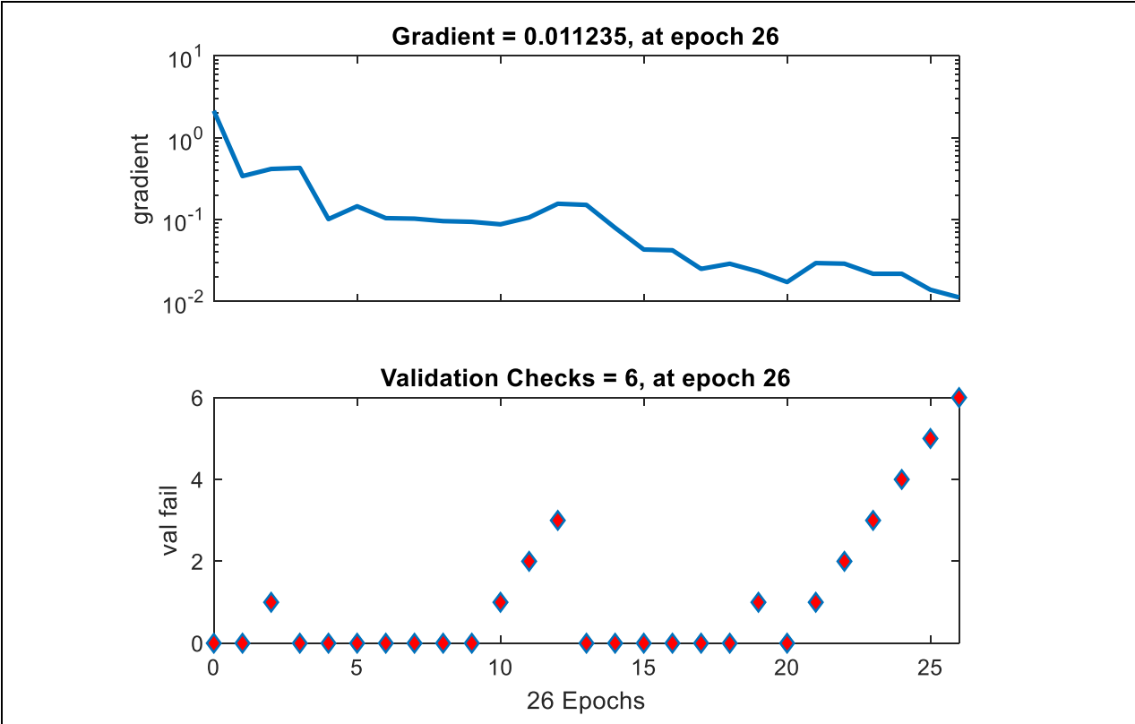
Figure 8. Results of the ANN gradient and val-fail training state.
