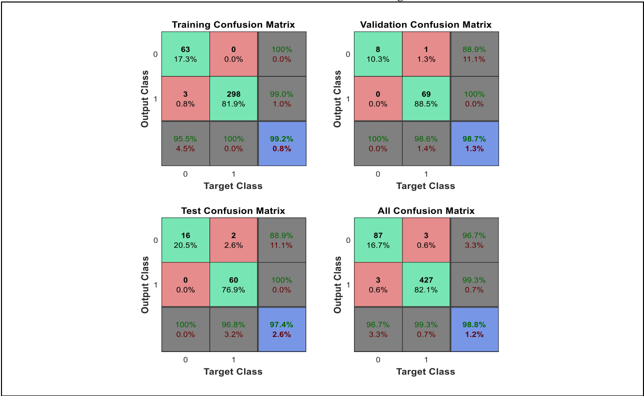
Figure 10. Confusion matrices of the training, validation, and test training.
