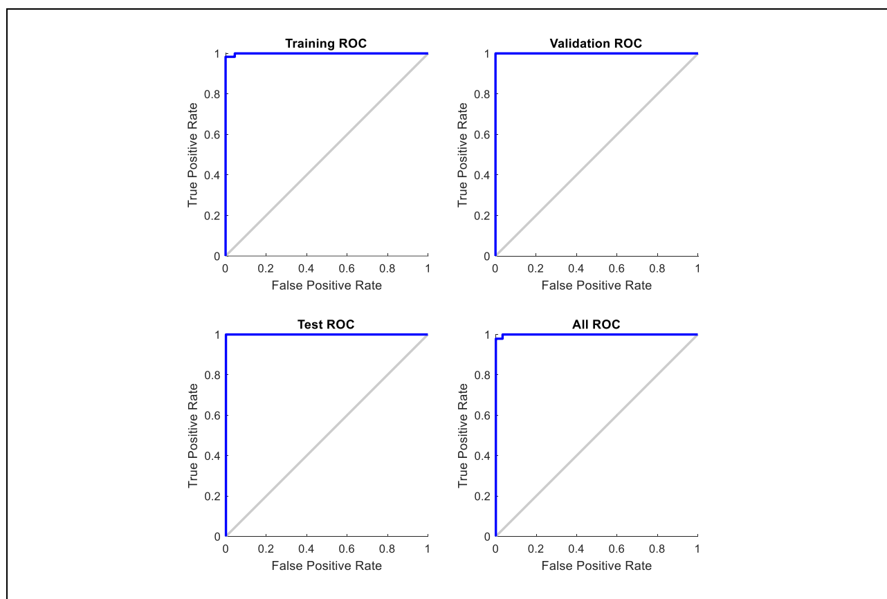
Figure 11: Results of the ANN receiver operating characteristics
