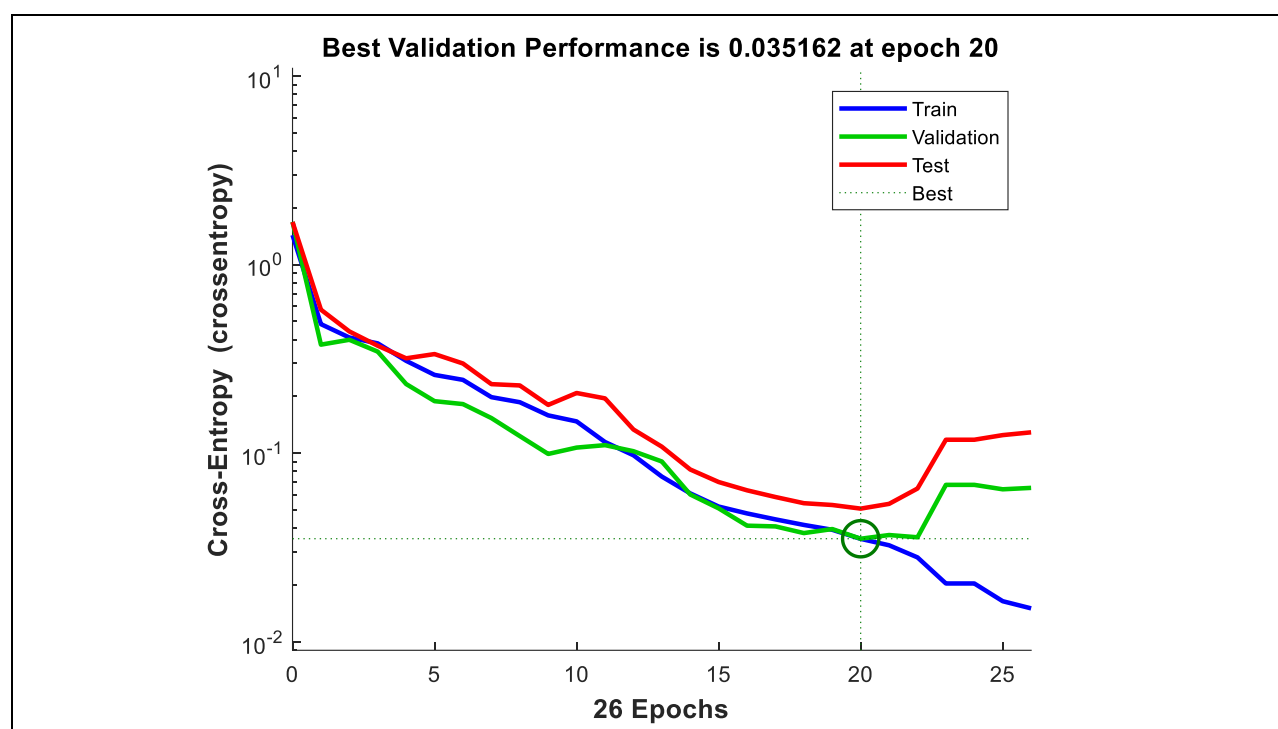
Figure 7. Results of the ANN test signals Cross-Entropy performance.
