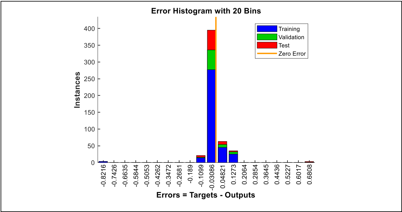
Figure 9. Results of the ANN error histogram.
